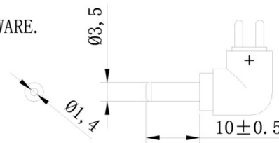
6. DETACHABLE PLUG. BLUE PLASTIC RING HARDWARE. Ø1. 40x3. 50x10. 0±0.5mm, "L"TYPE. USED 30P BLACK COLOR PVC.
