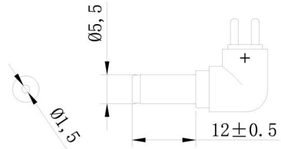
1. DETACHABLE PLUG. BLACK PLASTIC RING HARDWARE. Ø1. 50x5. 50x12. 0±0.5mm, "L"TYPE. USED 30P BLACK COLOR PVC.
