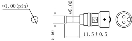
4. DETACHABLE PLUG. YELLOW PLASTIC RING HARDWARE. \varnothing 1.00 (pin) \times 5.00 \times 11.5 \pm 0.5 mm "I" type. used 20P black color PVC.
