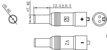
2. DETACHABLE PLUG. BLACK PLASTIC RING HARDWARE. \varnothing 0.60 \times 7.40 \times 12.5 \pm 0.5 mm "I" type. Used 20p black color pvc. (QV2) 270k 1/8W resistance
