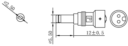
1. DETACHABLE PLUG. BLACK PLASTIC RING HARDWARE. \varnothing 2.50 \times 5.50 \times 12 \pm 0.5 mm "I" fork type. Used 20P black color PVC.
