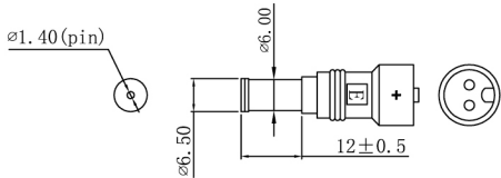
5. DETACHABLE PLUG. BLACK PLASTIC RING HARDWARE. \varnothing 1.40 (pin) \times 6.50 \times 12 \pm 0.5 mm "I" type. used 20P black color PVC.
