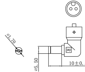
8. DETACHABLE PLUG. BLACK PLASTIC RING HARDWARE. \varnothing 1.70 \times 5.50 \times 10 \pm 0.5 mm "L" type. Used 20P black color PVC.
