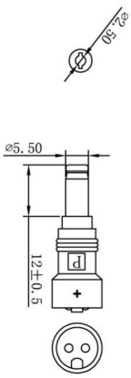
1. DETACHABLE PLUG, BLACK PLASTIC RING HARDWARE. \varnothing 2.50 \times 5.50 \times 12 \pm 0.5 mm "I" fork type. Used 20P black color PVC.
