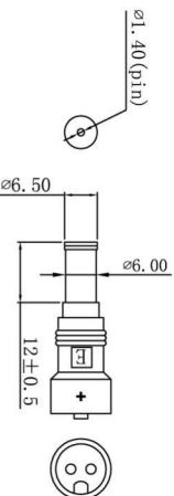
5. DETACHABLE PLUG, BLACK PLASTIC RING HARDWARE. \varnothing 1.40 (pin) \times 6.00 \times 12 \pm 0.5 mm "I" type. used 20P black color PVC.
