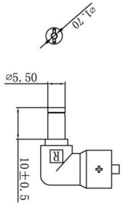
8. DETACHABLE PLUG, BLACK PLASTIC RING HARDWARE. \varnothing 1.70 \times 5.50 \times 10 \pm 0.5 mm "L" type. Used 20P black color PVC.
