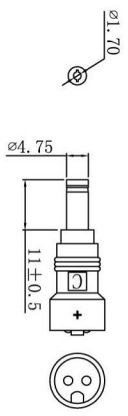
7. DETACHABLE PLUG, YELLOW PLASTIC RING HARDWARE. \varnothing 1.70 \times 4.75 \times 11 \pm 0.5 mm "I" type. used 20P black color PVC.
