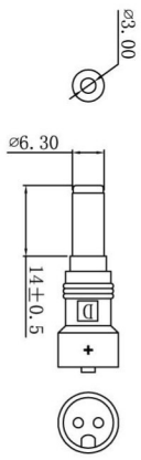
6. DETACHABLE PLUG, BLACK PLASTIC RING HARDWARE. \varnothing 3.00 \times 6.30 \times 14 \pm 0.5 mm "I" type. used 20P black color PVC.
