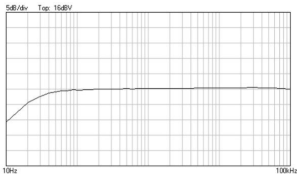
Frequentierespons @ 8 ohm
