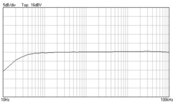
Frequenzgang @ 8 Ohm
